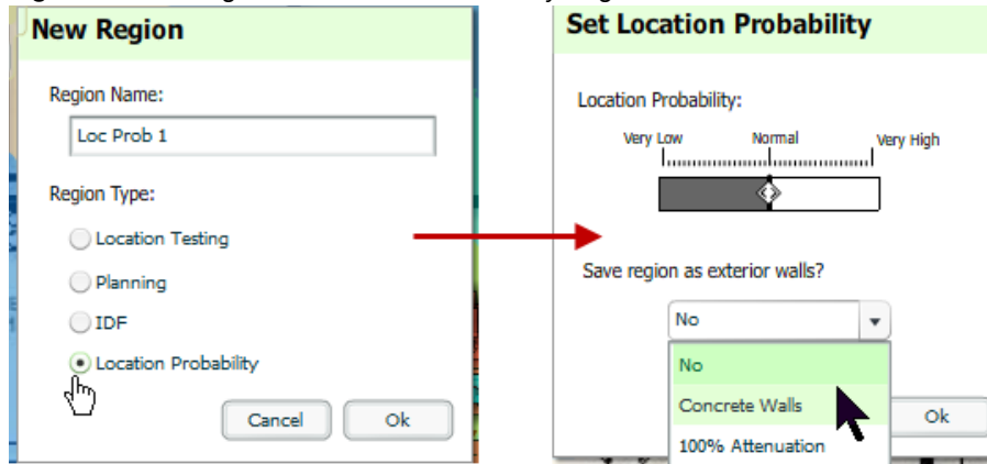
Figure 212 Adding a New Location Probability Region
