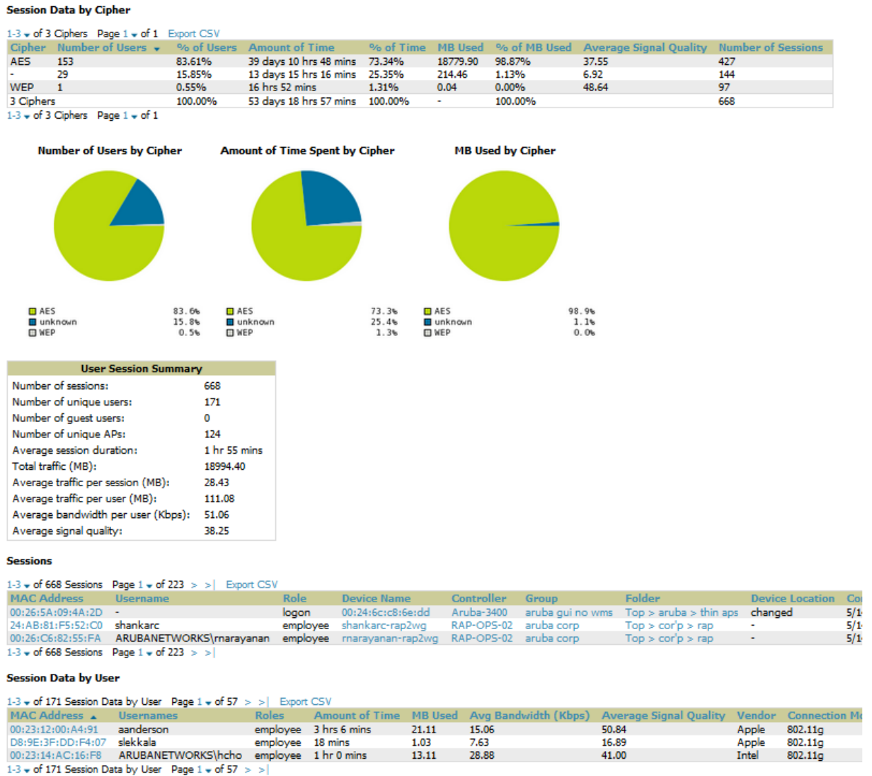
Figure 187 User Session Detail, Partial View
