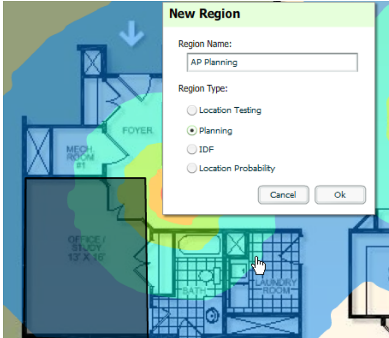
Figure 237 Planning Region Drawing and Selection Illustration
