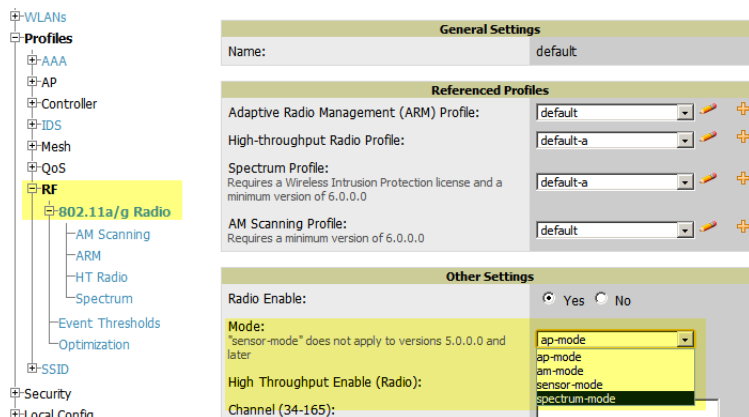
Figure 109 Spectrum mode in Alcatel-Lucent Configuration
